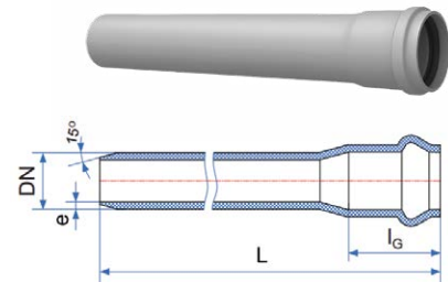
Ống nong gioăng (Rubber Ring Joint Pipe)
